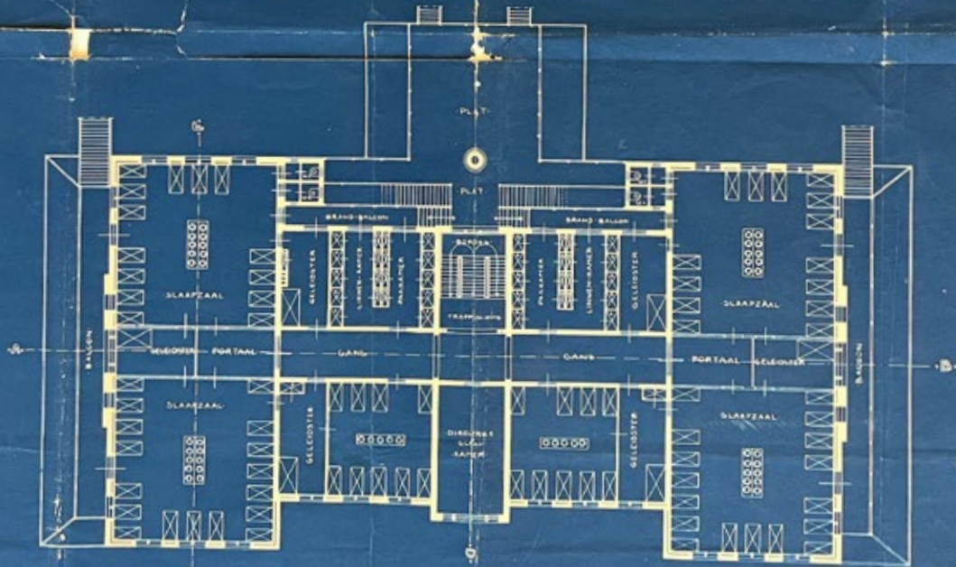
PLAN II - VANDIEPING
